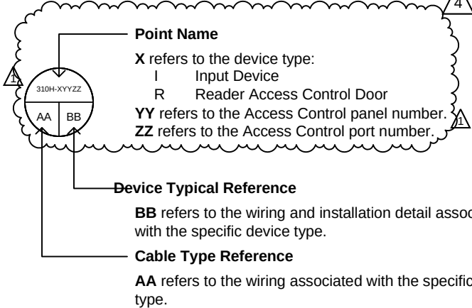
Access Control System Device Labeling
