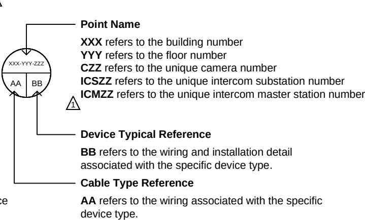
Video Surveillance and Intercom System Device Labeling
